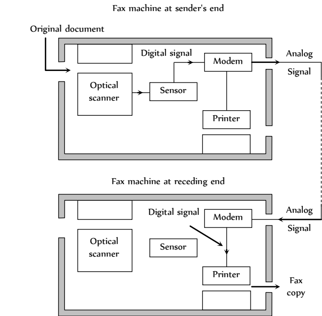
The original written document is put into the machine. A scanner scans the whole document. Fig. 28.20
